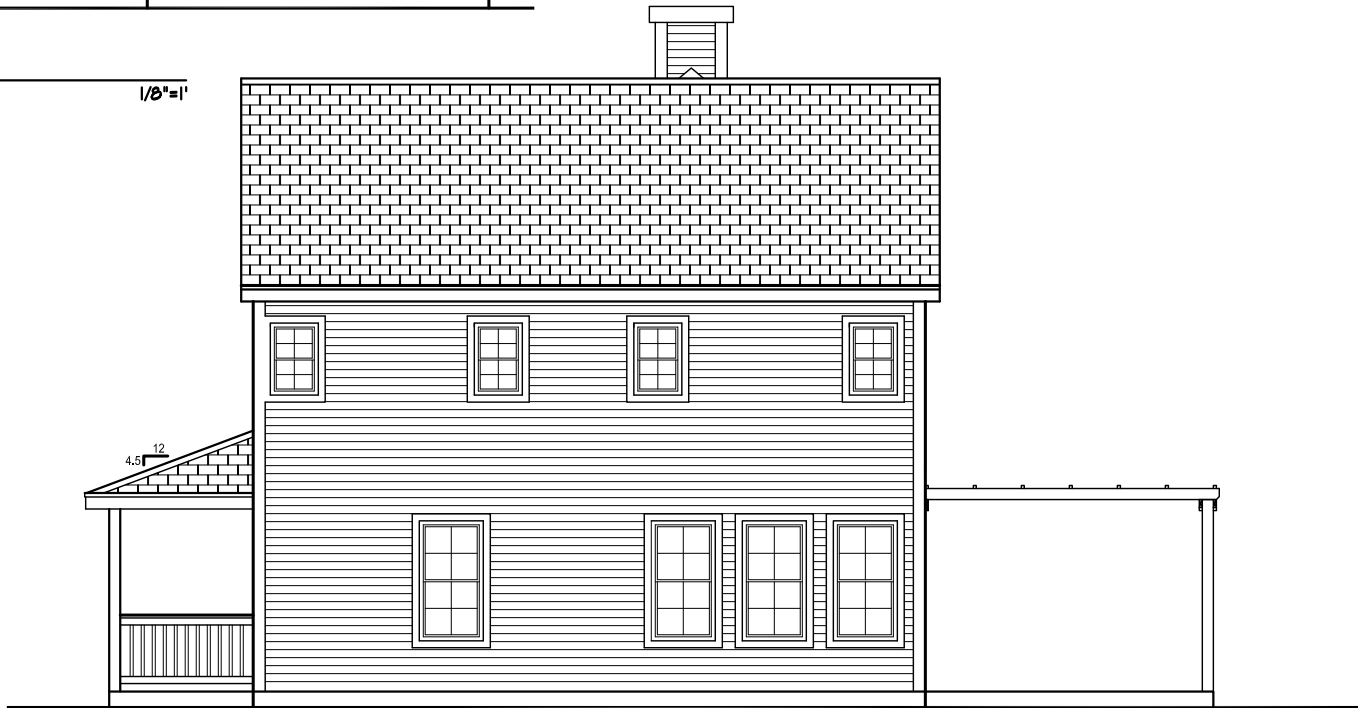
01 BACK ELEVATION
