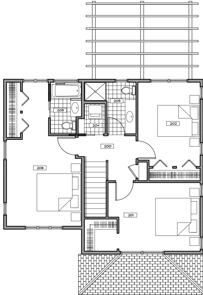
○ SECOND FLOOR PLAN 1/8"=1'
